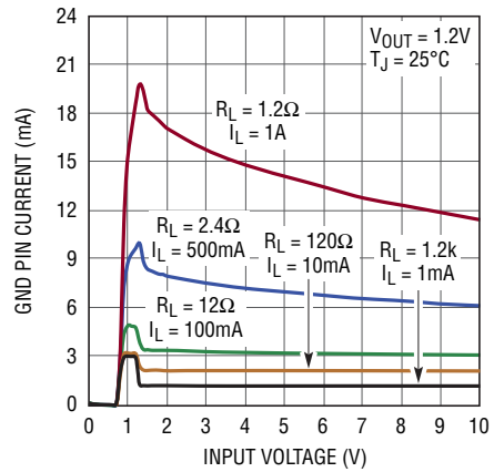
GND Pin Current
